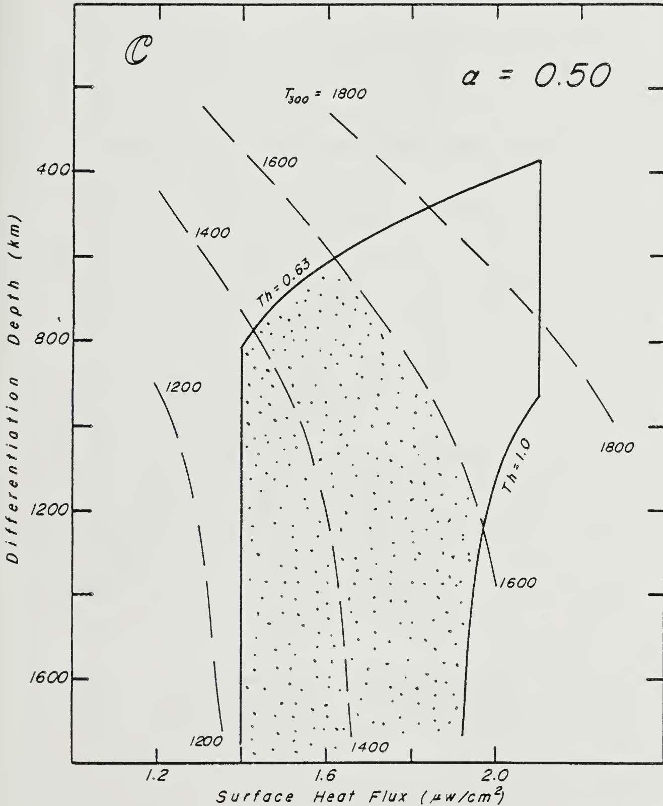
Three hundred kilometer temperature contours plotted versus average surface flux ( F_s ) and differentiation depth. The stippled area describes the range of 300 km temperatures and differentiation thicknesses which satisfy the heat flow and crustal thorium abundance data and the subsolidus requirement. The three sets of contours are distinguished by the assumed differentiation efficiency, \alpha : (a) \alpha = 1.0 ; (b) \alpha = 0.75 ; (c) \alpha = 0.50 .
